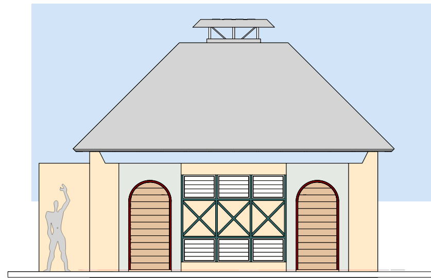
4 FACADE SUD 1:100
